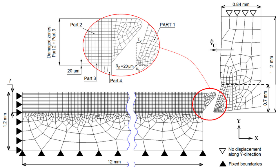
Fig. 9. Grid model and boundary conditions [33].
