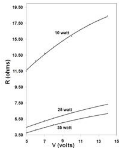
FIGURE 1. Resistance versus voltage curves obtained with 10 W, 25 W and 35 W incandescent lamps.
