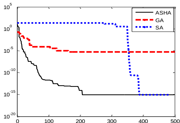
Figure 2: Iterative convergence on Ackley function.
