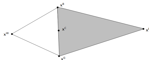
Fig 2: Expansion for Nelder- Meed Simplex Method
