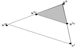
Fig 5: Shrink for Nelder- Meed Simplex Method 2.2 Hook- Jeeves Method
