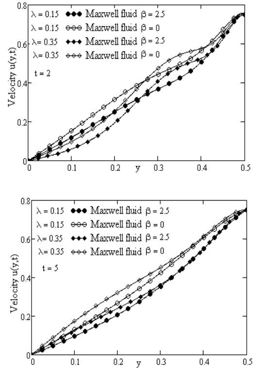
Fig. 2. Velocity profiles for Couette flows of Maxwell fluids ( V = 0.75, \nu = 0.35 )
